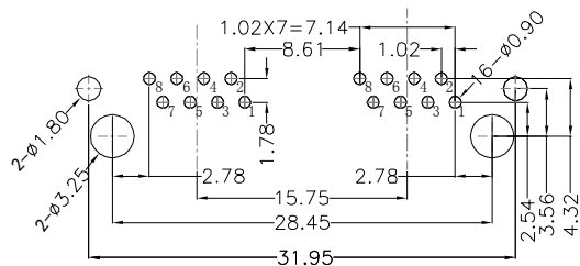
RECOMMENDED PCB LAYOUT VIEWED FROM COMPONENT SIDE
